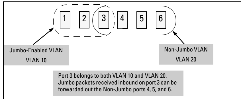
Figure 10-14. Forwarding Jumbo Packets Through Non-Jumbo Ports
