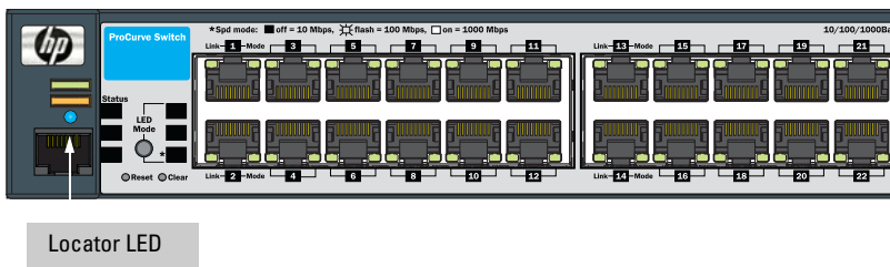
Figure B-25. Location of the Locator LED
